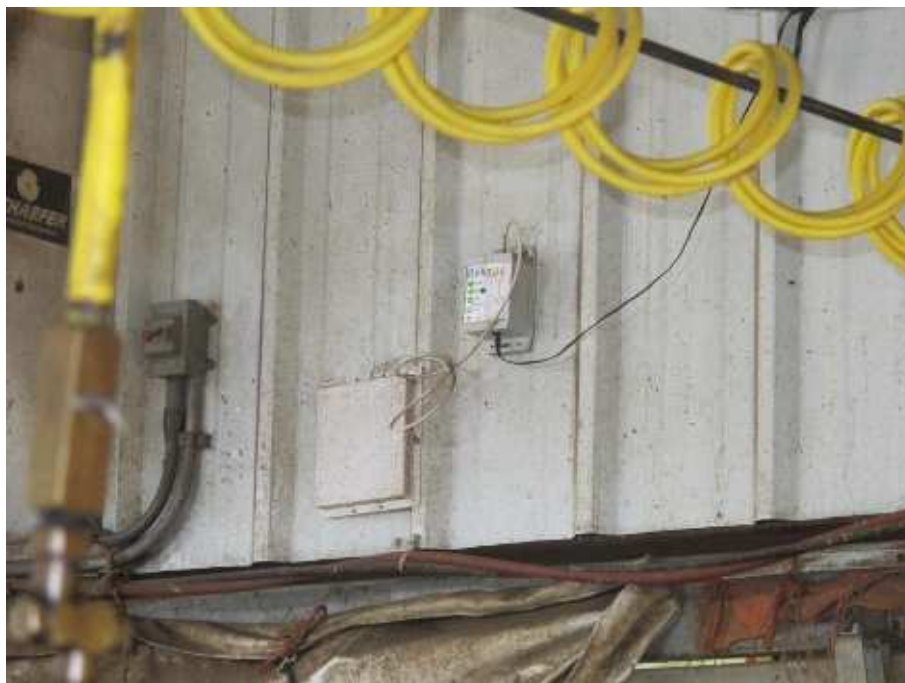
Figure 59: A BellaAg data receiver in the collecting yard
