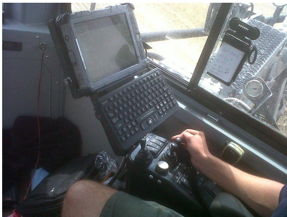
13 GPS grade control cab station, USA
