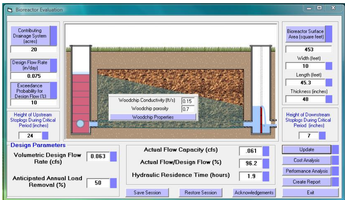
Subsurface Bioreactor evaluation guide
